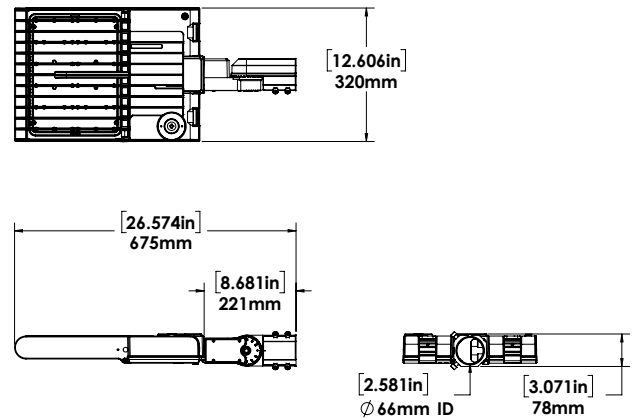
SLIP FITTER MOUNT
