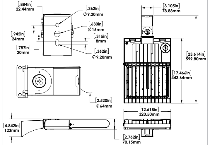
MOUNTING ARM
