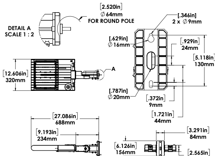
SLIP FITTER WITH WALL ADAPTOR MOUNT
