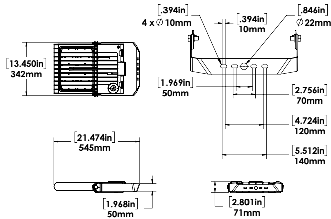
YOKE MOUNT
