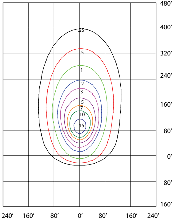
SFL2-LED600-H-4K-60DEG-BLK-DIM MOUNTED AT 50 FEET 50 DEGREE TILT
