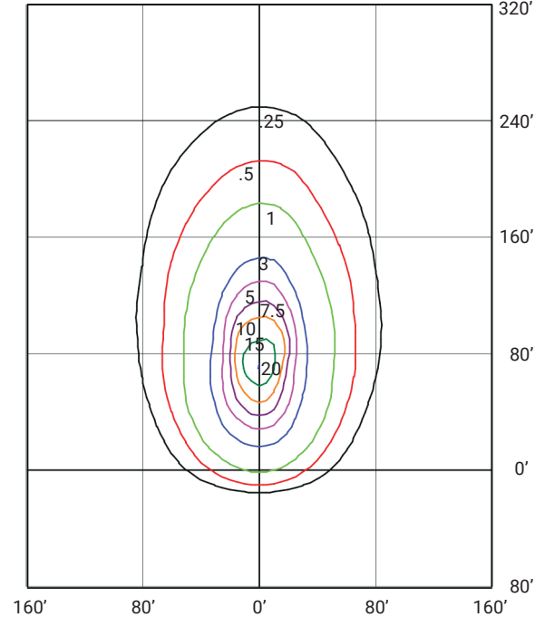
STRIKE1-LED600A400-B-5K-20DEG (600W, 5000K) 60 DEGREE TILT MOUNTED AT 50 FEET
