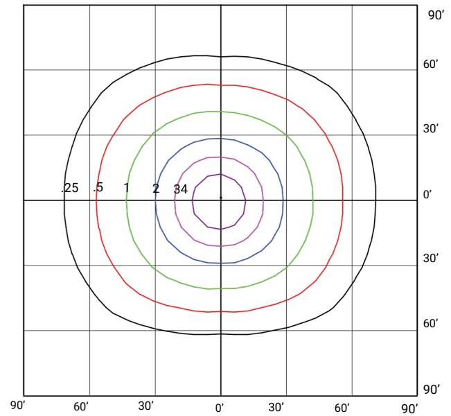
HELIX1-LED150A100-H-VK-T5-BRZ-DIM-SP10 (150W, 120V, 4000K) MOUNTED AT 30 FEET
