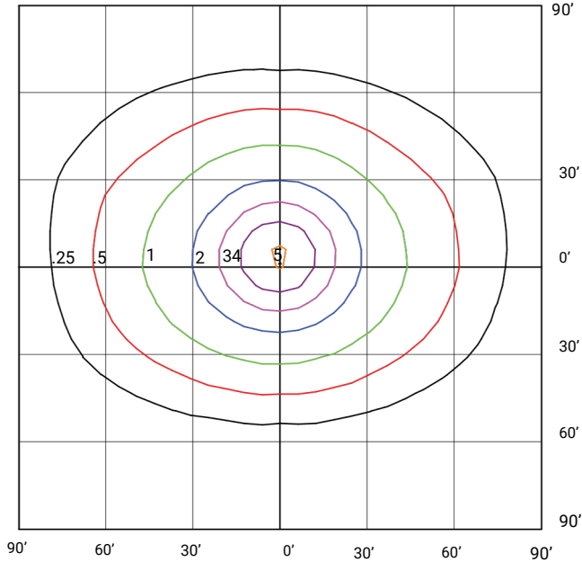
HELIX1-LED150A100-H-VK-T4-BRZ-DIM-SP10 (150W, 120V, 4000K) MOUNTED AT 30 FEET
