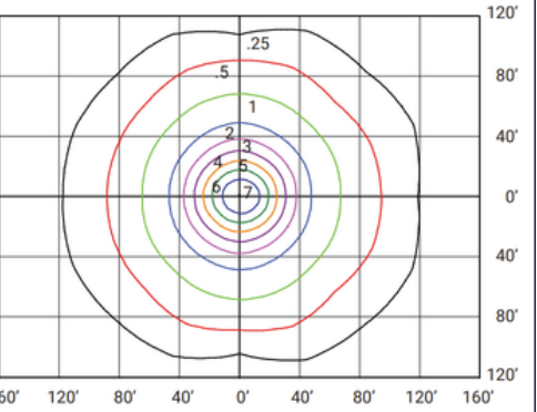
JAG3S-LED430A300-H-VK-VD1-BRZ-DIM-PC-SP10 (430W, 5000K, TYPE V) MOUNTED AT 40 FEET
