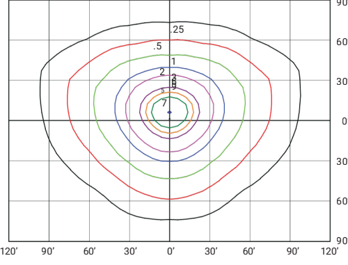
JAG2S-LED240A180-H-VK-VD1-BRZ-DIM-SP10 (240W, 4000K, TYPE IV) MOUNTED AT 30 FEET
