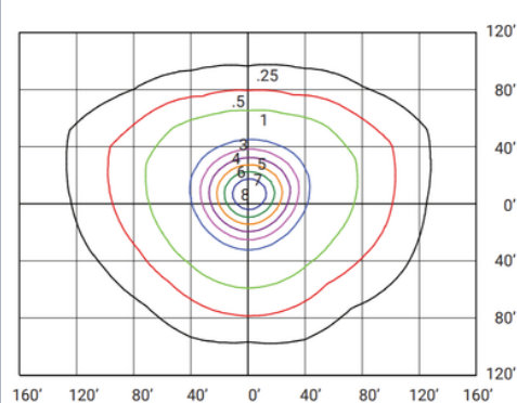
JAG3S-LED430A300-H-VK-VD1-BRZ-DIM-PC-SP10 (430W, 5000K, TYPE IV) MOUNTED AT 40 FEET
