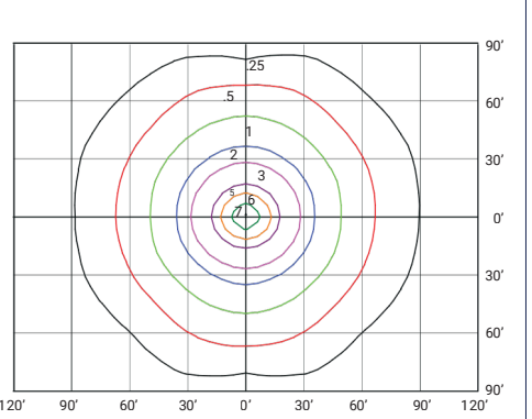
JAG2S-LED240A180-H-VK-VD1-BRZ-DIM-SP10 (240W, 4000K, TYPE V) MOUNTED AT 30 FEET
