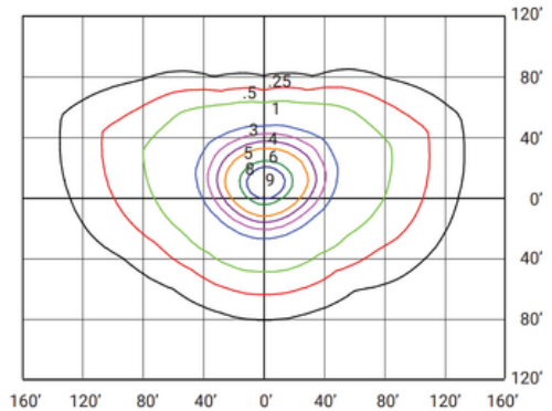
JAG3S-LED430A300-H-VK-VD1-BRZ-DIM-PC-SP10 (430W, 5000K, TYPE III) MOUNTED AT 40 FEET
