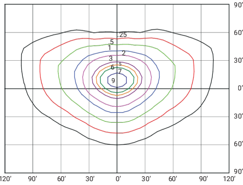
JAG2S-LED240A180-H-VK-VD1-BRZ-DIM-SP10 (240W, 4000K, TYPE III) MOUNTED AT 30 FEET
