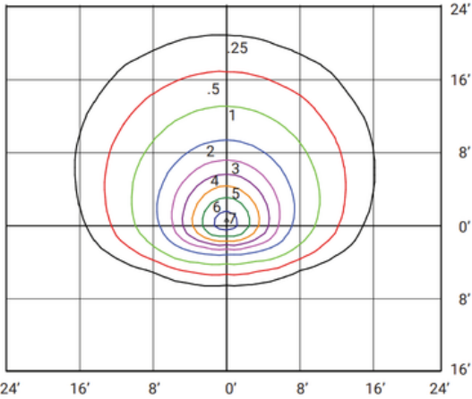
FL3-LED50A30-B-VK-BRZ-DIM-PC (120V 50W 5000K) MOUNTED AT 15 FEET WITH 30 DEGREE TILT
