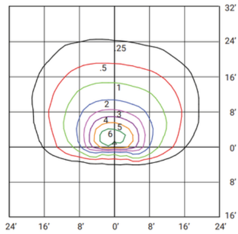
FL2-LED30A15-B-VK-BRZ-DIM-PC (120V 30W 5000K) MOUNTED AT 15 FEET WITH 45 DEGREE TILT
