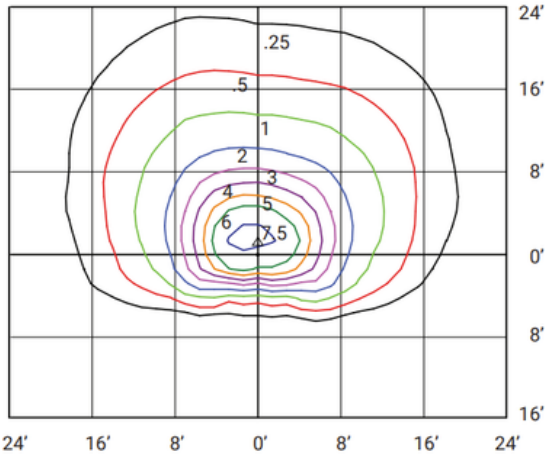
FL2-LED30A15-B-VK-BRZ-DIM-PC (120V 30W 5000K) MOUNTED AT 15 FEET WITH 30 DEGREE TILT
