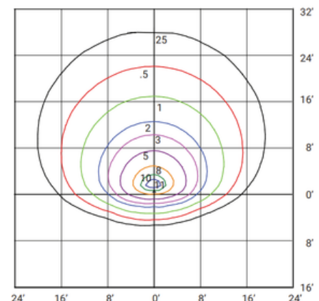
FL3-LED50A30-B-VK-BRZ-DIM-PC (120V 50W 5000K) MOUNTED AT 15 FEET WITH 45 DEGREE TILT
