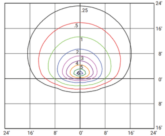
FL3-LED50A30-B-VK-BRZ-DIM-PC (120V 50W 5000K) MOUNTED AT 15 FEET WITH 45 DEGREE TILT
