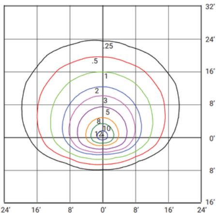
FL3-LED50A30-B-VK-BRZ-DIM-PC (120V 50W 5000K) MOUNTED AT 15 FEET WITH 30 DEGREE TILT
