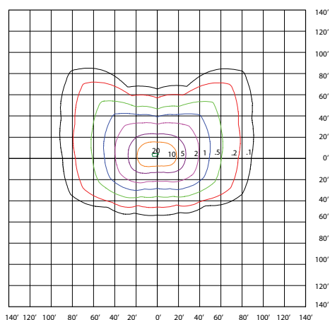
FL8A-LED300 TYPE IV / 7H X 7V
