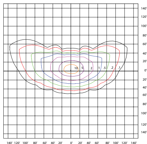
FL8A-LED300 TYPE III / 7H X 7V
