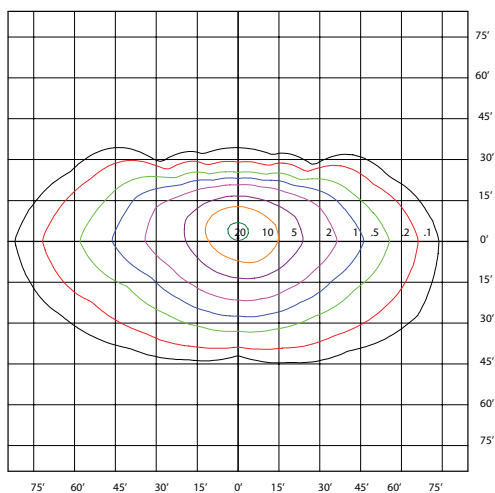
FL8A-LED300 TYPE II / 7H X 6V
